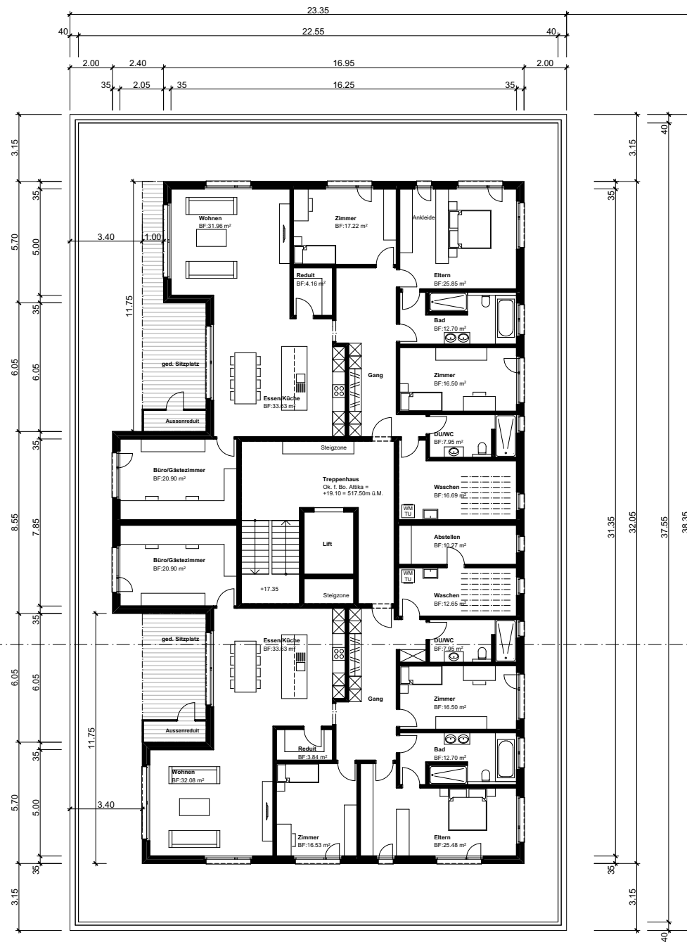
Grundriss Attika
